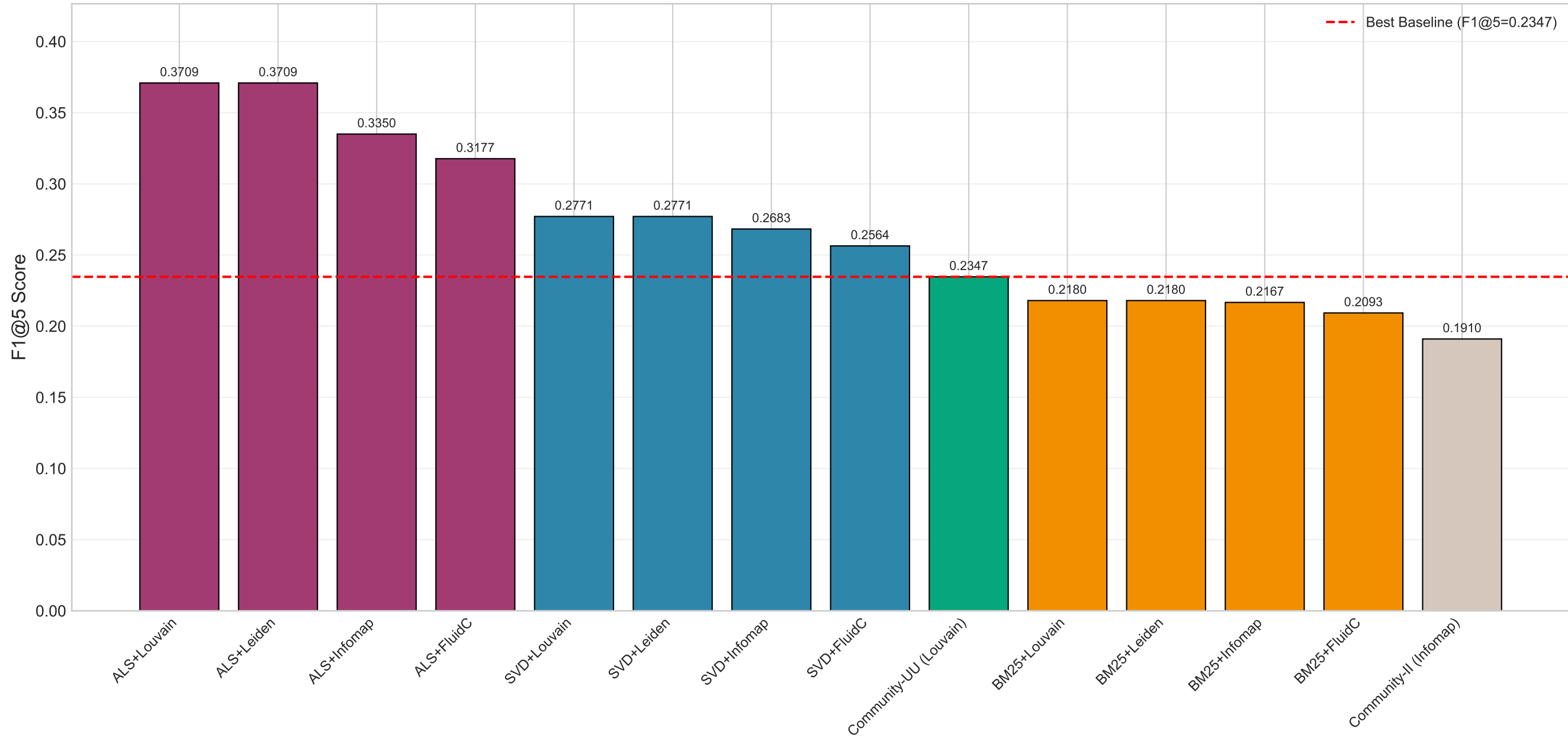
Figure 33: F1@5 Comparison of All Recommender Approaches
